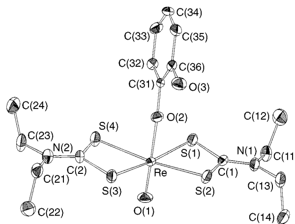
Fig. 1 Perspective view of [\text{ReO}\{\text{O}(\text{OH})\text{C}_6\text{H}_4\}(\text{S}_2\text{CNET}_2)_2] 1 showing the atom labelling scheme
